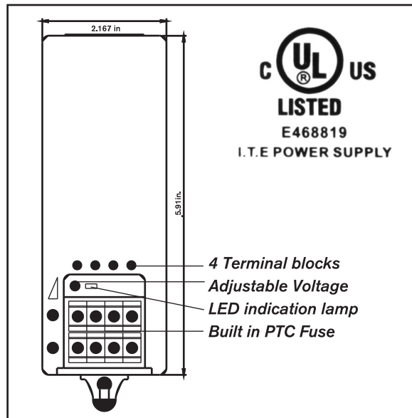
4 Output – 12VDC/5AMP – 13.8VDC/4.3AMP Camera Power Supply – Model VT-1205A-D4K
