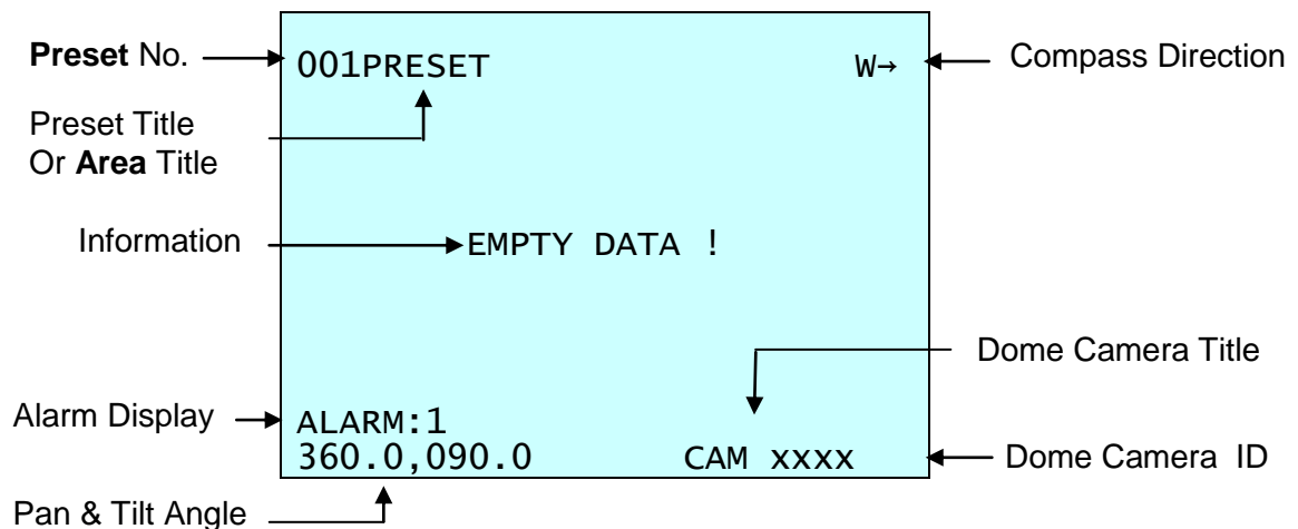
On Screen Display in normal control mode
