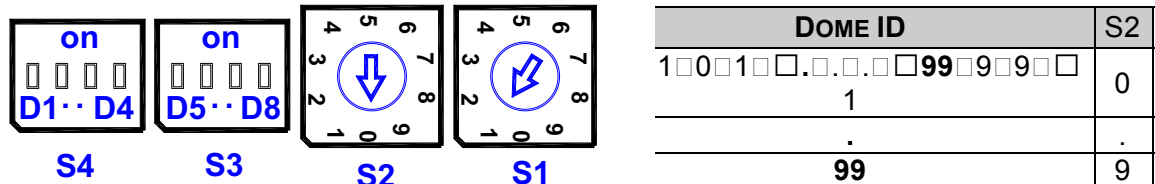
Figure 9 - Setting Dome Camera Address (ID) and Protocol
